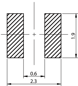
Land Pattern: [mm]
