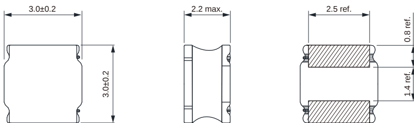
Dimensions: [mm]
